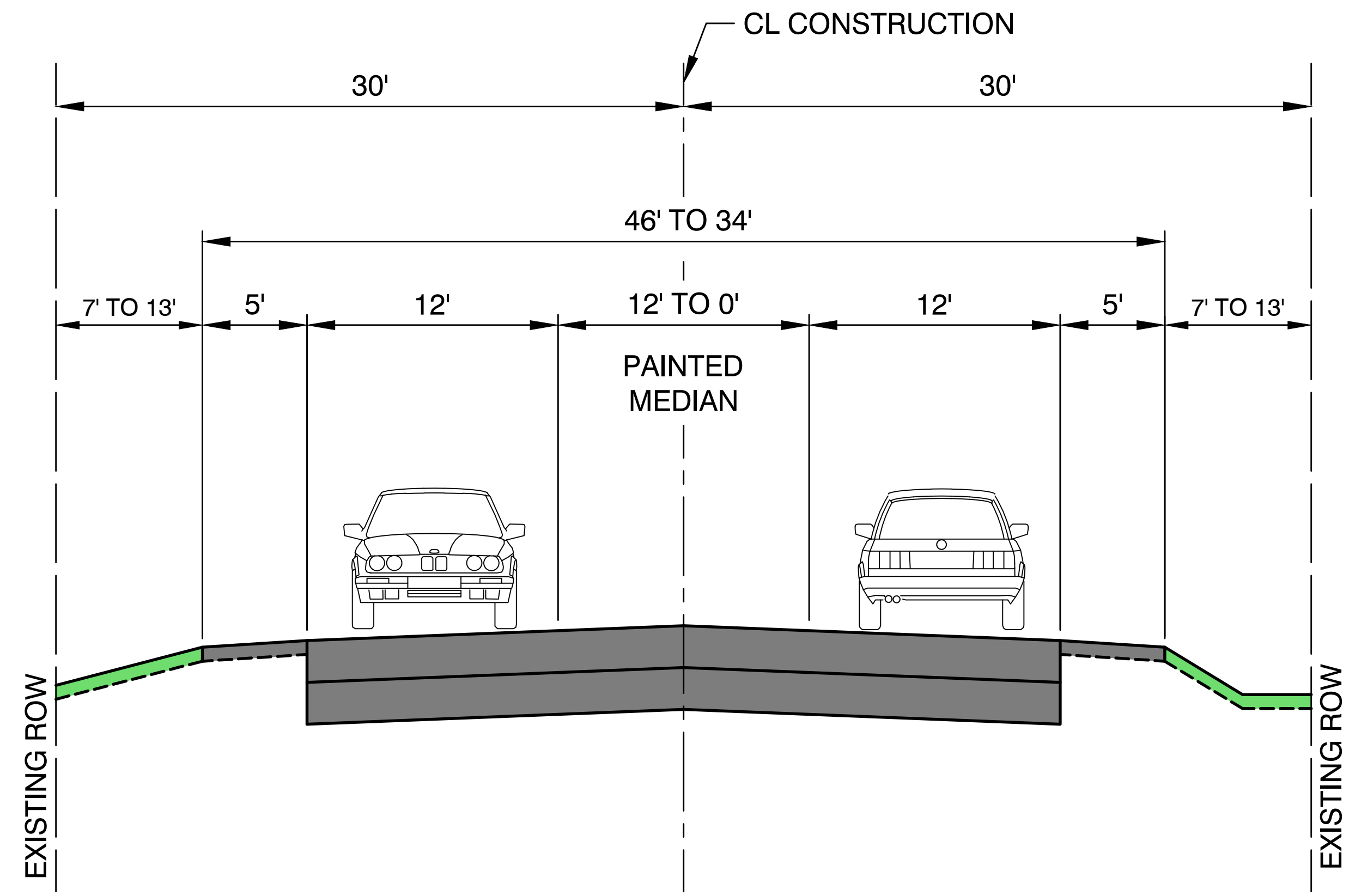
PROPOSED OAK FOREST AVENUE EAST OF RIDGELAND AVENUE
