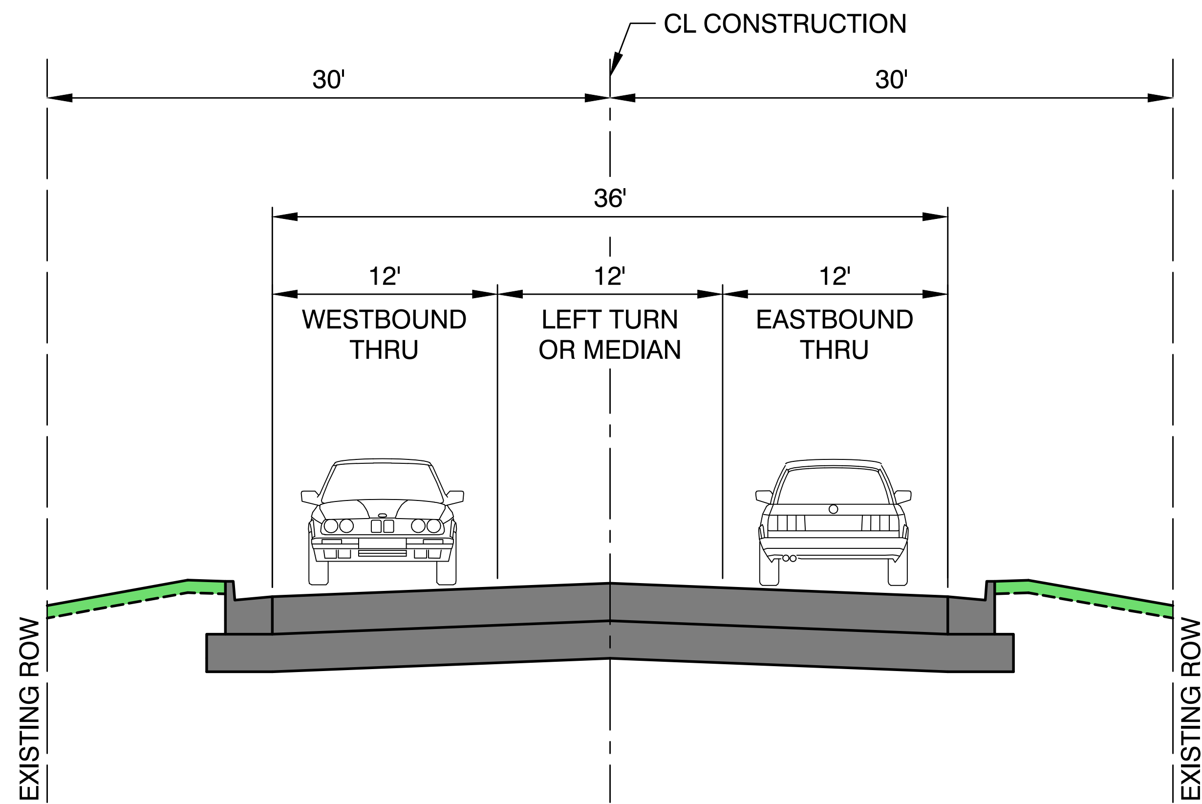
PROPOSED OAK FOREST AVENUE AT RIDGELAND AVENUE
